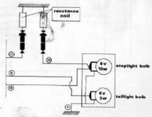
Wiring diagram in alternative with "ULO" tail/stop light unit (2 bulbs).
